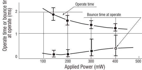
OPERATE TIME
