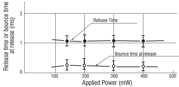
RELEASE TIME
