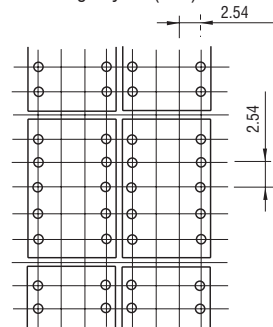
Mounting Layout (mm)
