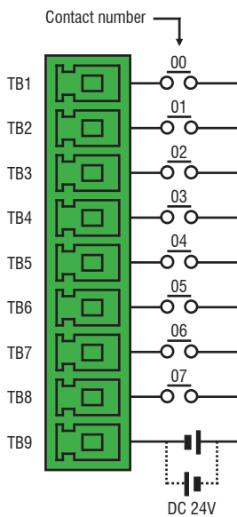
8 Point DC Input XBE-DC08A
