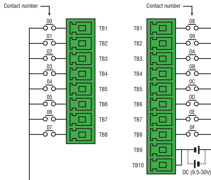
16 Point DC Input XBE-DC16B
